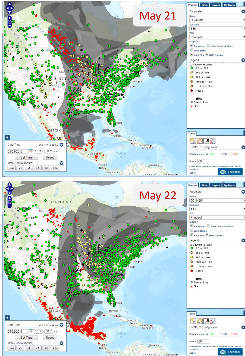
Figure showing location of fires and smoke (from HMS fire and smoke data) along with late afternoon ozone levels. Elevated ozone levels (yellow points) evident in Midwest/western Great Lakes region. Display generated via AirNow-Tech ( http://www.airnowtech.org/ )
