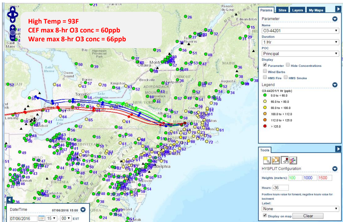
Figure showing late afternoon ozone levels in the northeast US on July 6, 2016. 36-hour back trajectories calculated with HYSPLIT model also overlaid on map showing air transport generally from the west to the Chicopee and Ware monitoring locations. Display generated via AirNow-Tech ( http://www.airnowtech.org/ )
