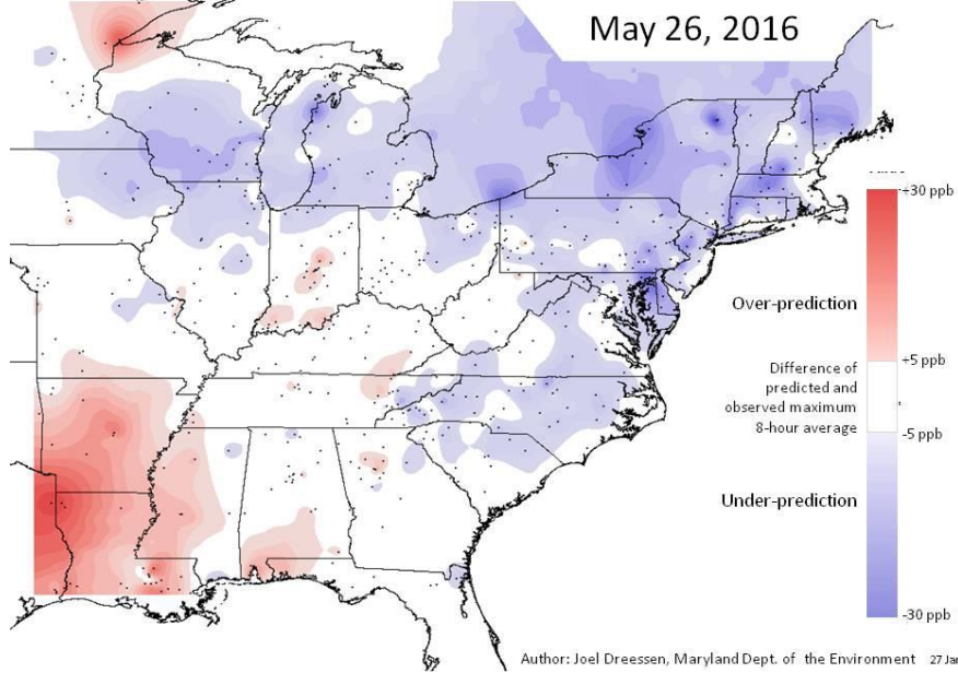
Figure showing CMAQ model bias to observed ozone levels. Blue shadings indicate degree of model under-prediction as smoke influences ozone levels across much of the northeast. Image courtesy of Joel Dreessen MDDEP.
