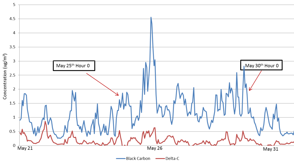
Figure 29 Springfield Hourly Black Carbon and Delta-C – May 21-31, 2016
