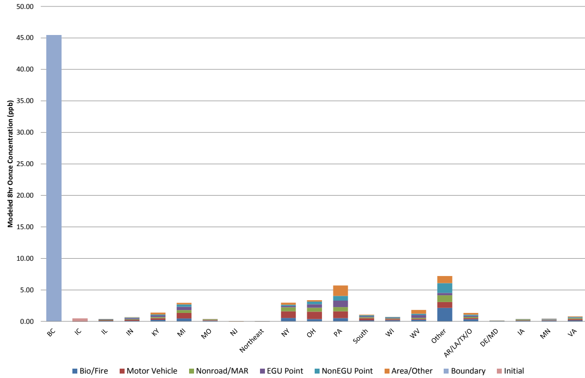
2018 OSAT Results - 75 ppb Threshold Day Average
